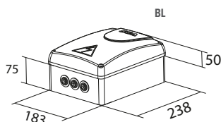
DIMENSIONS (mm)
