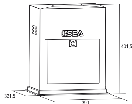
DIMENSIONS (mm)
